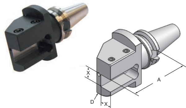
Tsugami 15T
